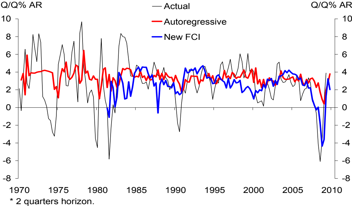
Figure 5.2: Real GDP Growth: Forecast using Autoregressive and New FCI Models (h=2)*
