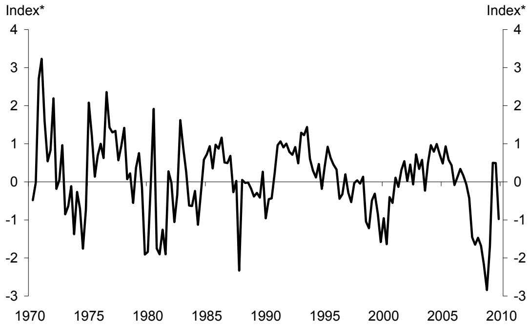
Figure 5.1: New FCI: First Principal Component of 44 Financial Indicators
