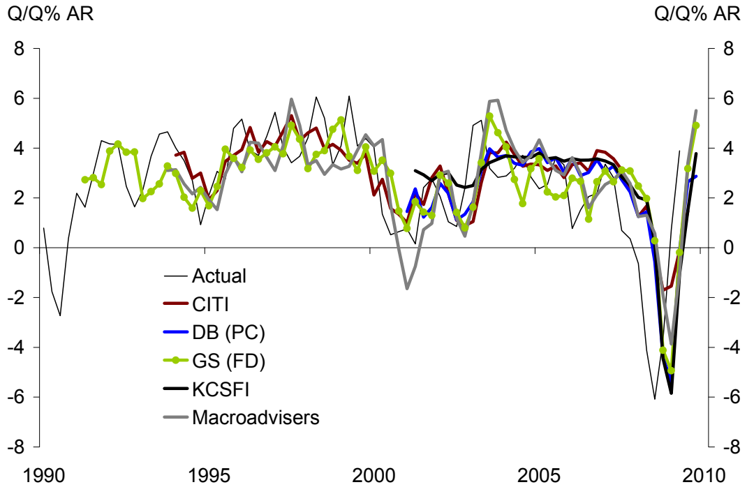
Figure 5.3 b. Real GDP Growth: Forecast using Alternative FCIs ( h=2 )*
