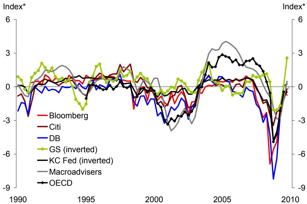
Figure 2.2 Seven Alternative Financial Conditions Indices
